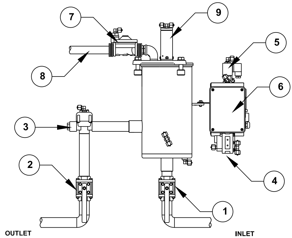
WITH C.O.V.
