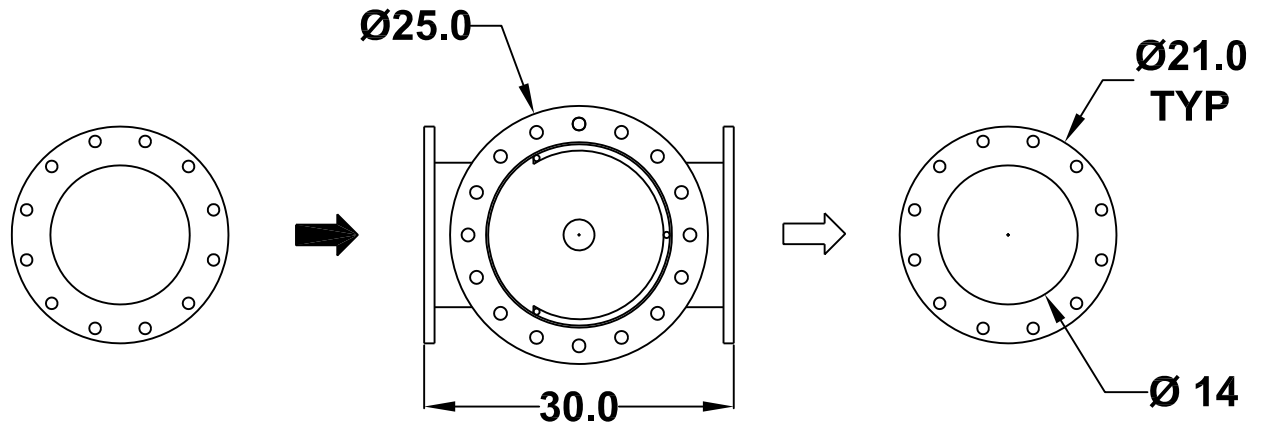
TOP VIEW WITH COVER REMOVED
